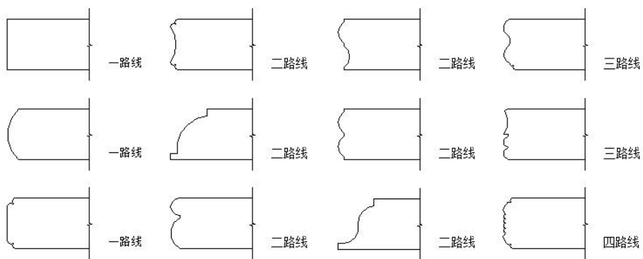
砖细线脚
